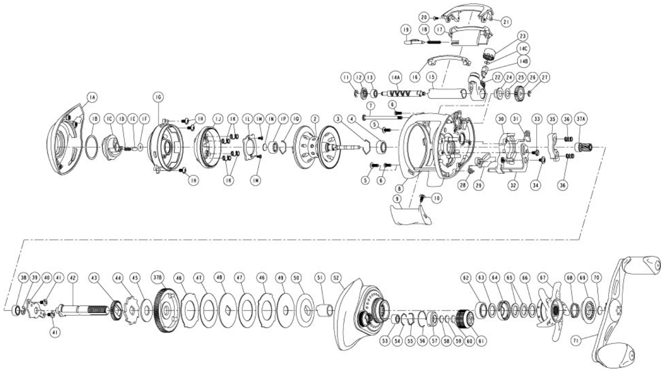
Quantum TKVD150SPT Baitcast Reel Part List
